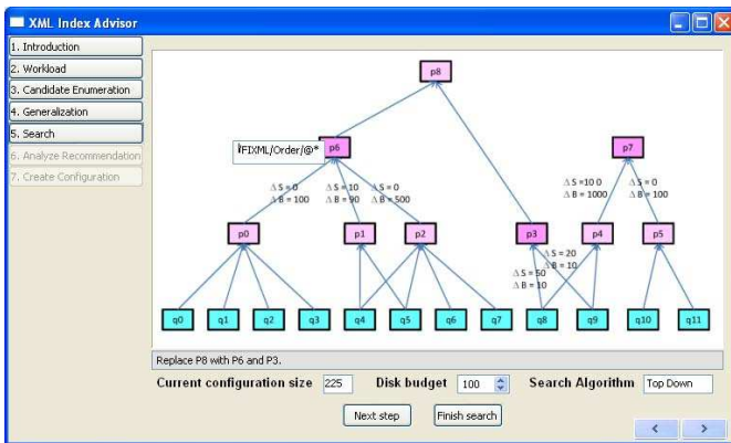
Figure 4: Searching the space of candidate indexes.
