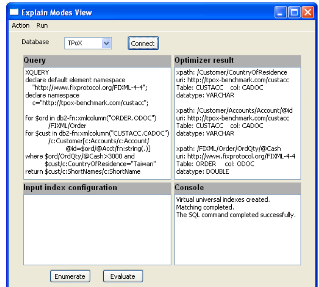
Figure 2: Basic candidate recommendation.
